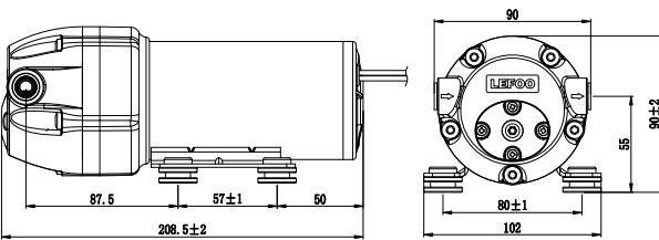
LFP1800J-V1、LFP2800J-V1 (3/8" TOP FEMALE QUICK CONNECTOR)
