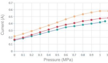
Current Curve
