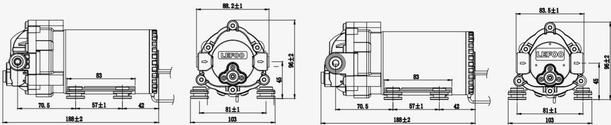
LFP6500W\6600WD\6800WD(5/16" Side female quick connector)
