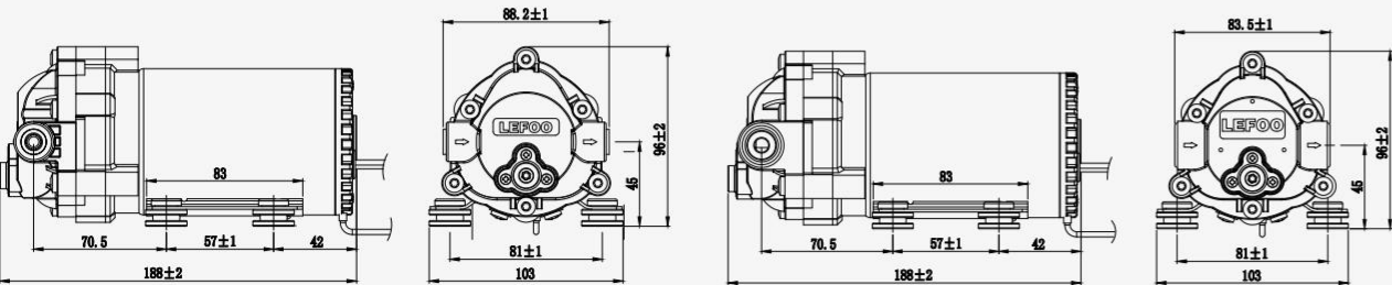
LFP6200WD\6300WD-A\6300WD\6400WD(5/16" Side female quick connector)
