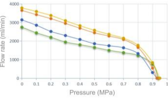
Flow Curve
