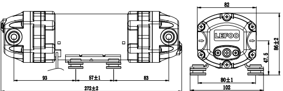
LFP21500J-FD (3/8" NPT)
