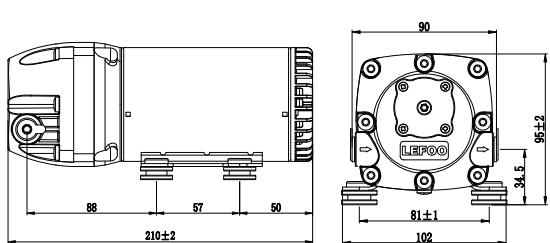
LFP21500W (3/8" SIDE FEMALE QUICK CONNECTOR)
