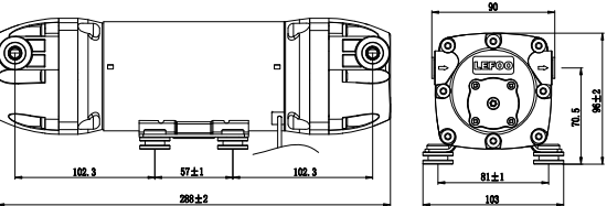
LFP21500W-FD (3/8" SIDE FEMALE QUICK CONNECTOR)
