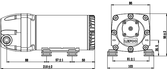
LFP21500W (3/8" NPT "0")
